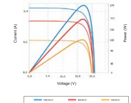
I-V Curves
